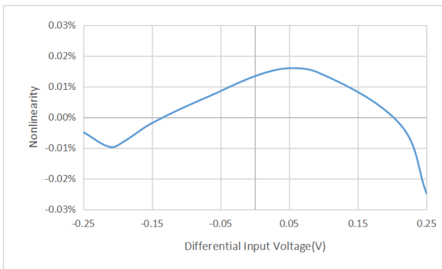
Figure 5.13 Nonlinearity vs Input Voltage (NSI1300D25)
