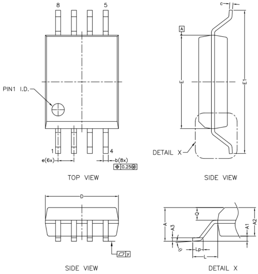
Figure 9.1 SOW8 Package Shape and Dimension in millimeters
