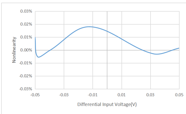
Figure 5.14 Nonlinearity vs Input Voltage (NSI1300D05)
