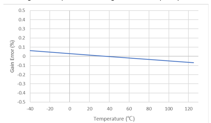
Figure 5.7 Gain Error vs Temperature
