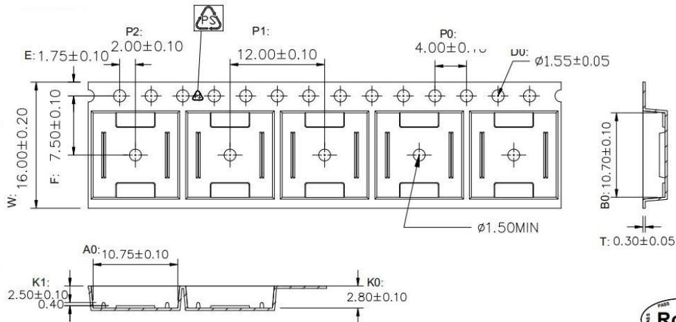
Figure 12.2 Reel Information of SOP8(300mil)
