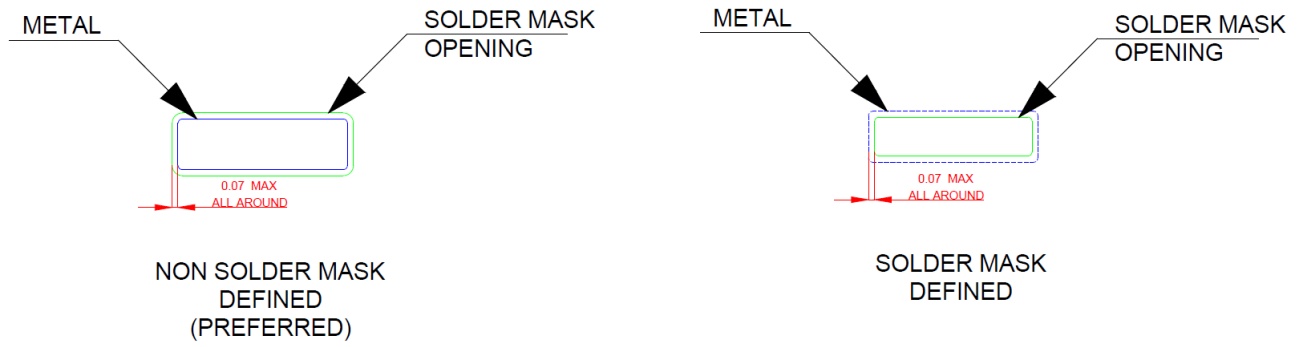
Figure 9.5 Solder Mask Details(mm)
