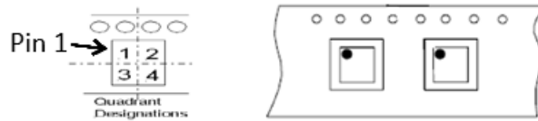
Figure 11.4 Quadrant Designation for Pin1 Orientation in Tape
