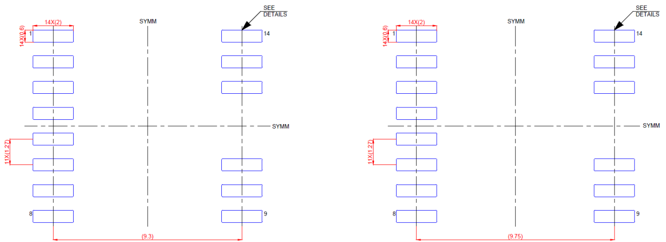
Figure 9.4 SOW14 Package Board Layout Example(mm)
