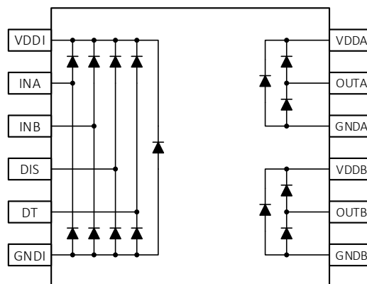
Figure 7.3 ESD Structure
