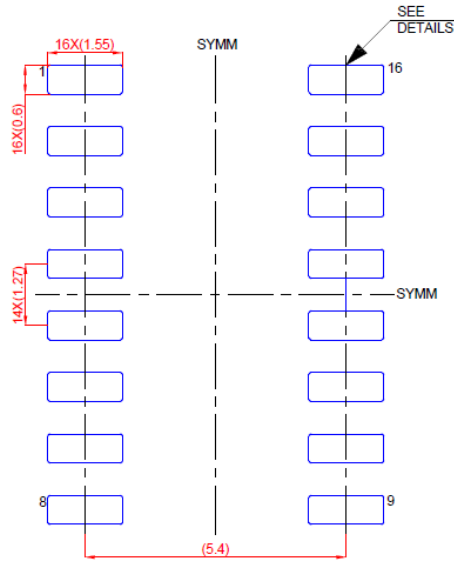
Figure 9.4 SOP16 Package Board Layout Example(mm)
