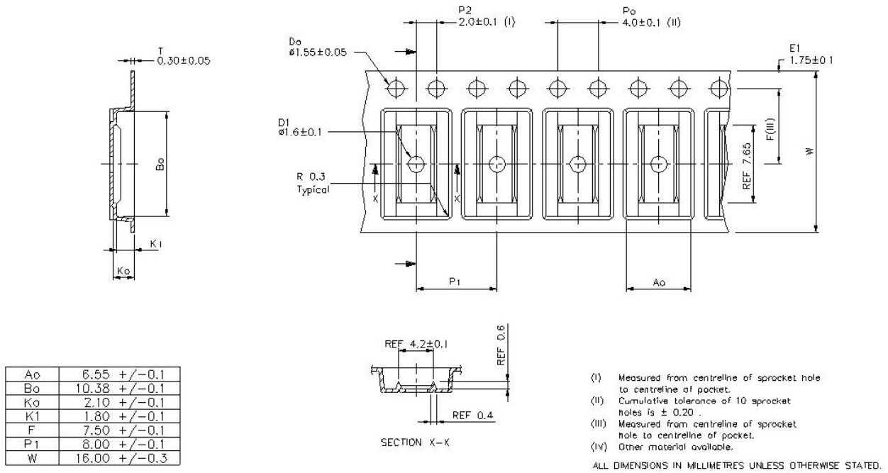
Figure 11.3 SOP16 Reel Information
