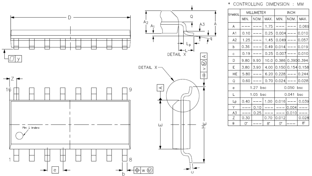
Figure 9.3 SOP16 Package Shape and Dimension
