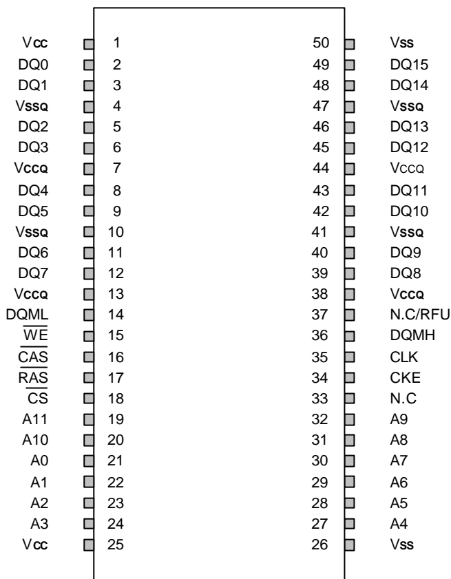
50-pin Plastic TSOP-II
