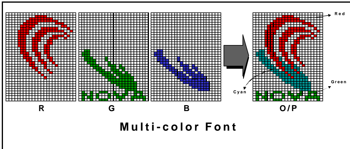
Figure 14. Multi-Color Font
