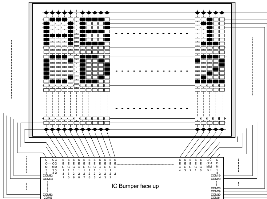
Type II (ADC=1, COM=1)
