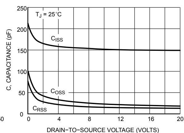
Figure 6. Capacitance Variation
