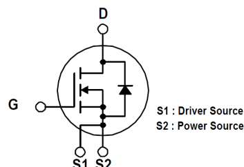
N-Channel MOSFET
