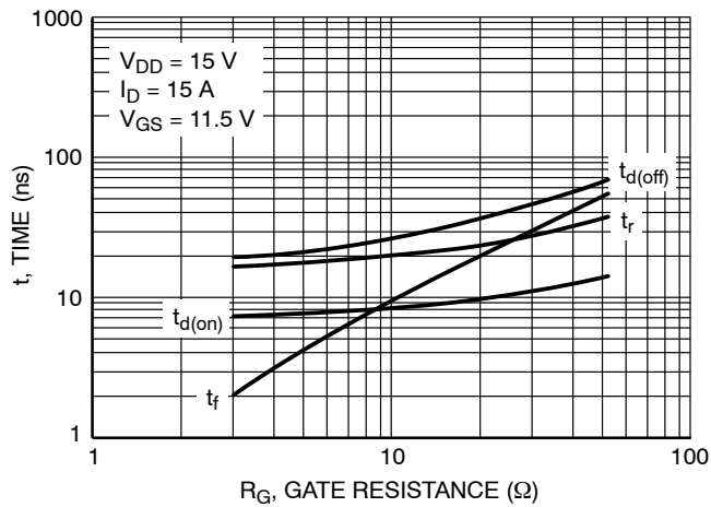
www.DataSheet4U.com Figure 9. Resistive Switching Time Variation vs. Gate Resistance
