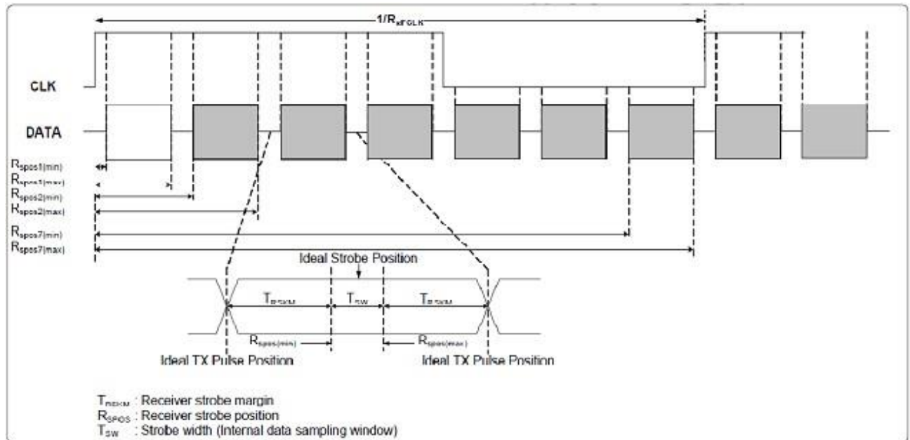
LVDS figure
