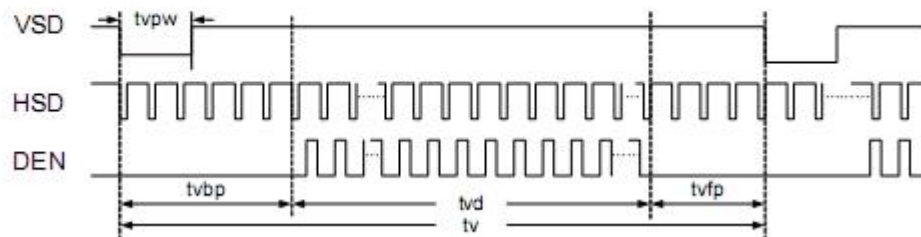
Vertical input timing diagram
