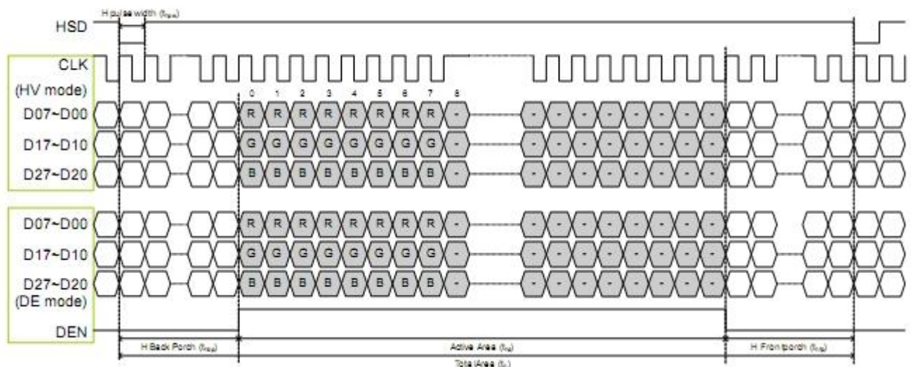
Horizontal input timing diagram
