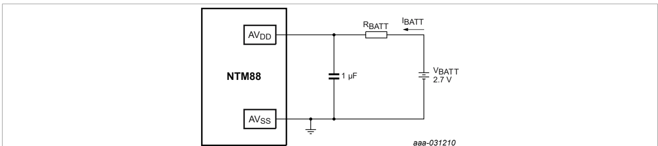
Figure 7. Battery performance test configuration
