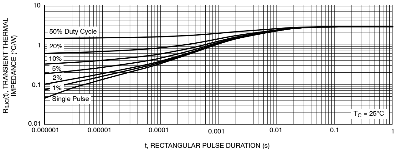
Figure 14. Thermal Response
