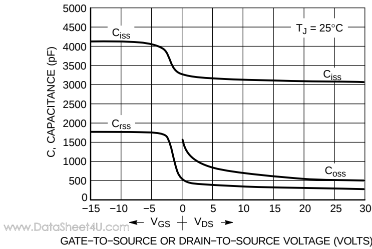
Figure 7. Capacitance Variation
