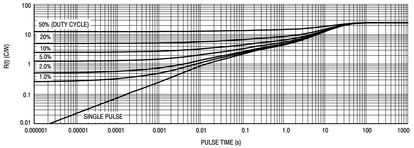
Figure 13. Thermal Impedance
