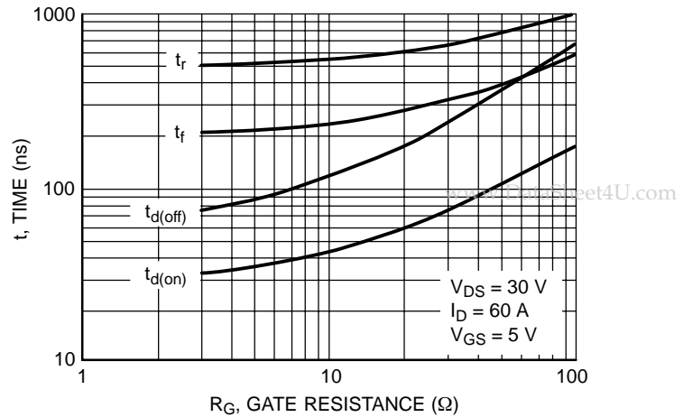
Figure 9. Resistive Switching Time Variation versus Gate Resistance
