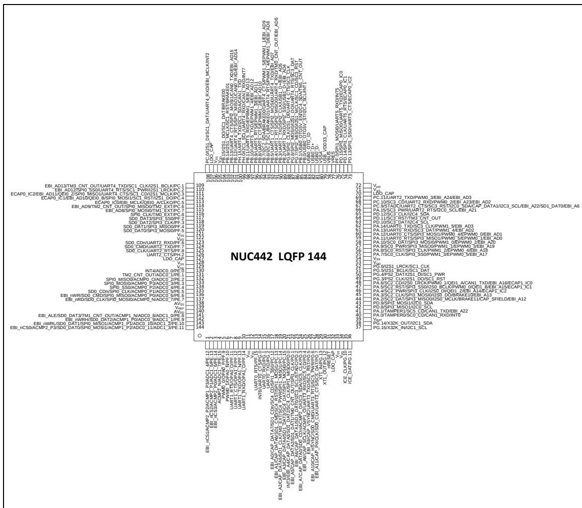
Figure 4.2-4 NuMicro™ NUC442Jxxxx LQFP 144-pin Diagram
