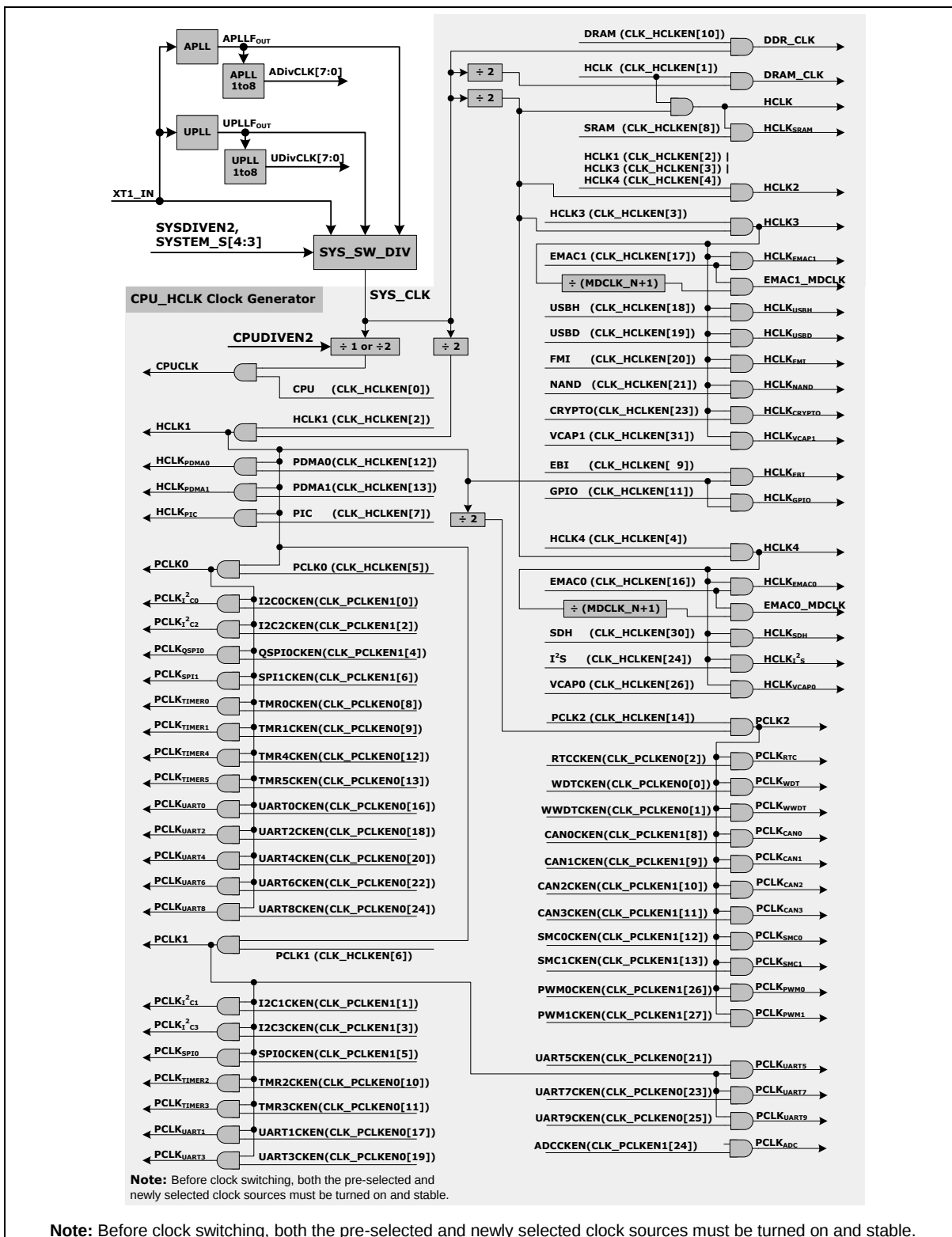
Figure 6.3-14 CPU_HCLK Clock Generator Block Diagram
