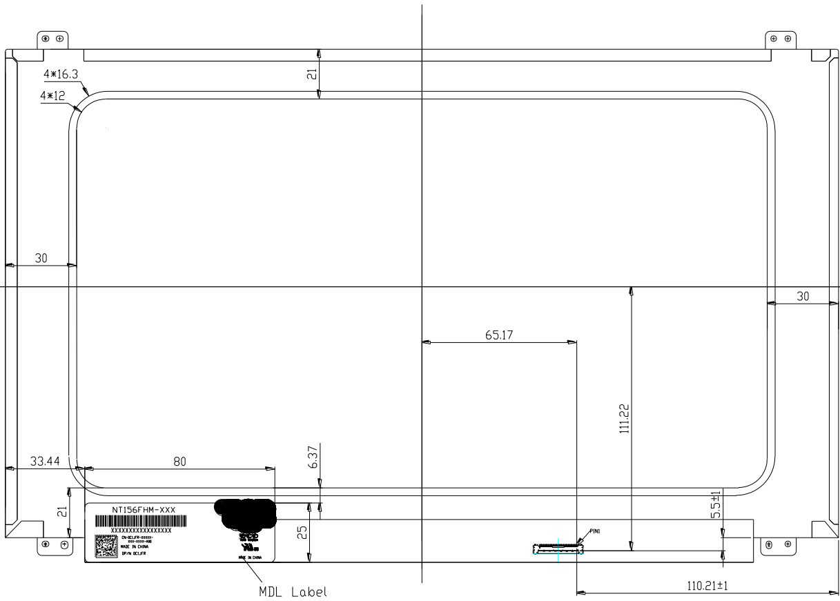
Figure 7. Outline Dimensions (Rear view)
