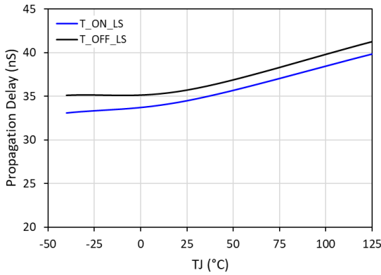
Fig. 17. Propagation delay ( T_{ON} and T_{OFF} ) vs. junction temperature ( T_J ) – low side
