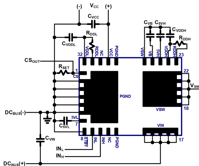
Fig. 24. IC connection diagram
