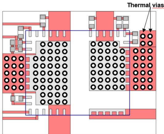
Step 3. Place many thermal vias inside source pad and inside source copper areas. (dia=0.65mm, hole=0.33mm, pitch=0.925mm, via wall=1mil)
