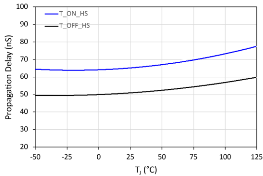
Fig. 17. Propagation delay ( T_{ON} and T_{OFF} ) vs. junction temperature ( T_J ) – low side
