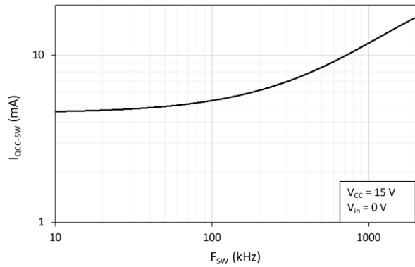
Fig. 14. V_{CC} operating current ( I_{QCC-SW} ) vs. operating frequency ( F_{SW} )
