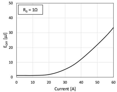
Fig. 16. E_{OFF} vs. I_{DS} , T_{JUNC} = 25\text{ °C}
