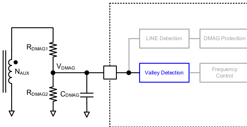
Figure 24 Valley Detection Circuit
