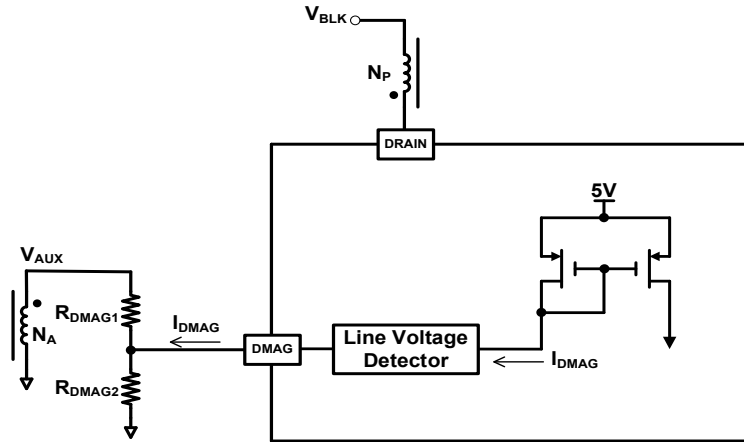
Figure 27 Line Voltage Detection Circuit
