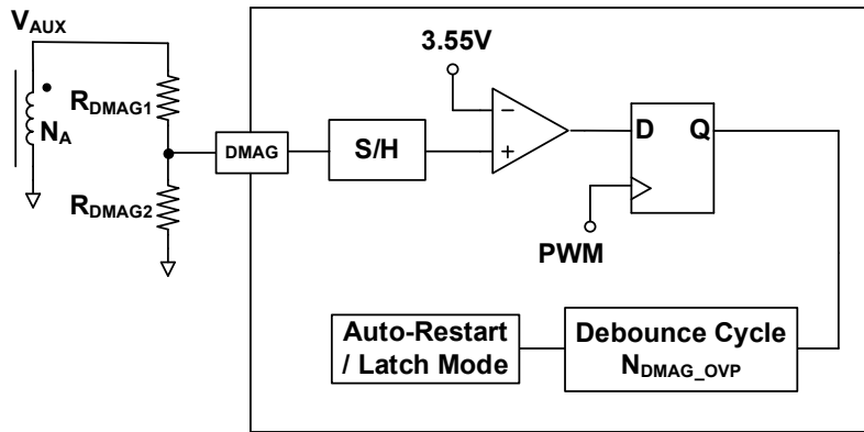
Figure 29 DMAG Over Voltage Protection Circuit
