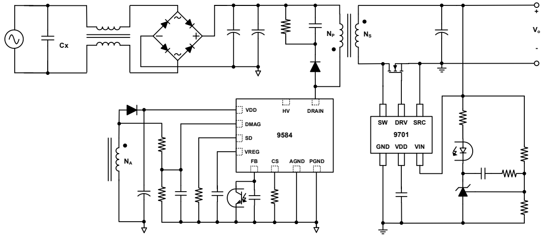
HFQR Flyback
