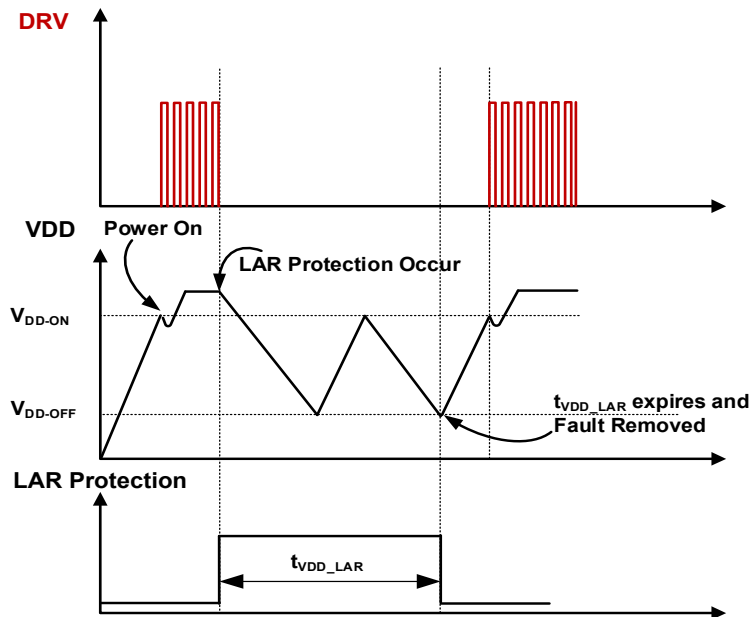
Figure 28 Auto-Restart Long AR Mode
