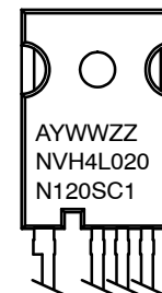
MARKING DIAGRAM
