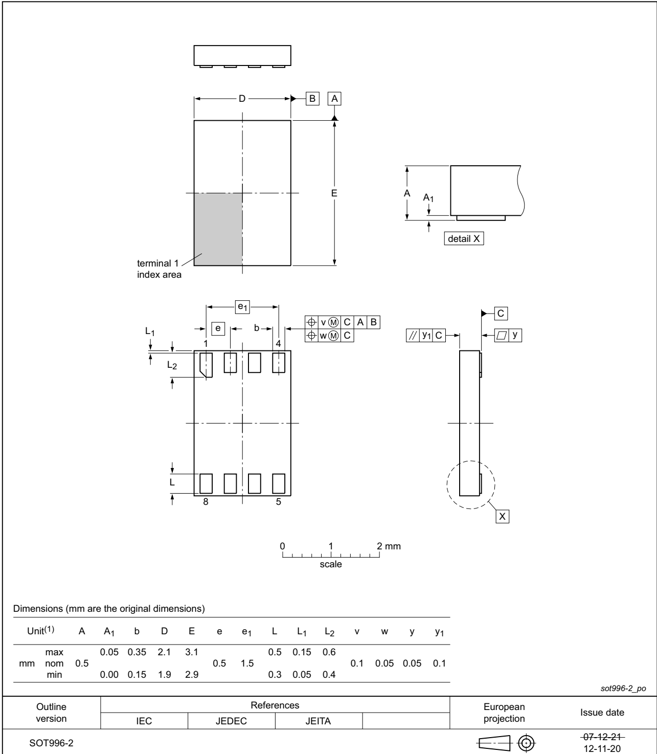
Fig 16. Package outline SOT996-2 (XSON8U)
