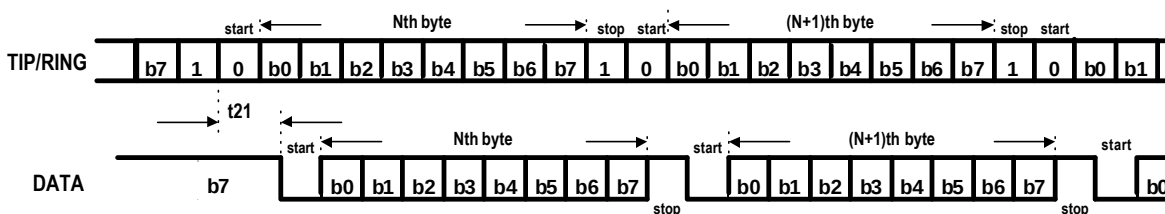
Figure 24. Serial Data Interface Timing in MODE '0'
