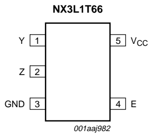
Fig 3. Pin configuration SOT353-1 (TSSOP5)
