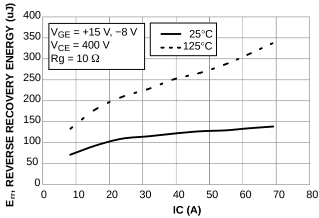
Figure 39. Typical Reverse Recovery Energy Loss vs. IC
