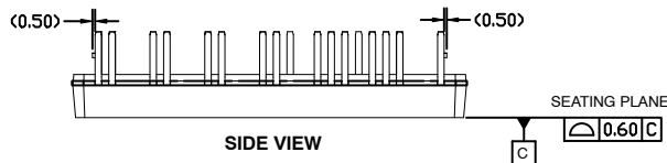
DIP27 73.2x40.2 CASE 184AA ISSUE B
