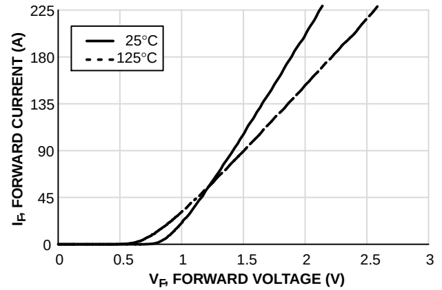
Figure 60. Converter Diode Forward Characteristics
