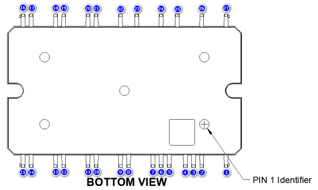
Figure 2. Pin Configuration
