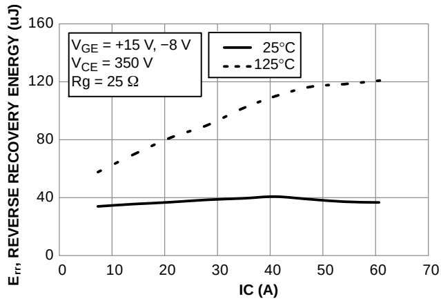
Figure 11. Typical Reverse Recovery Energy Loss vs. IC
