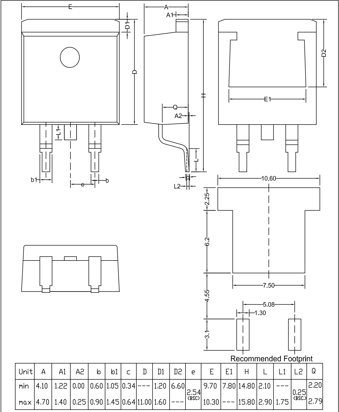
Fig. 8. Package outline TO263N
