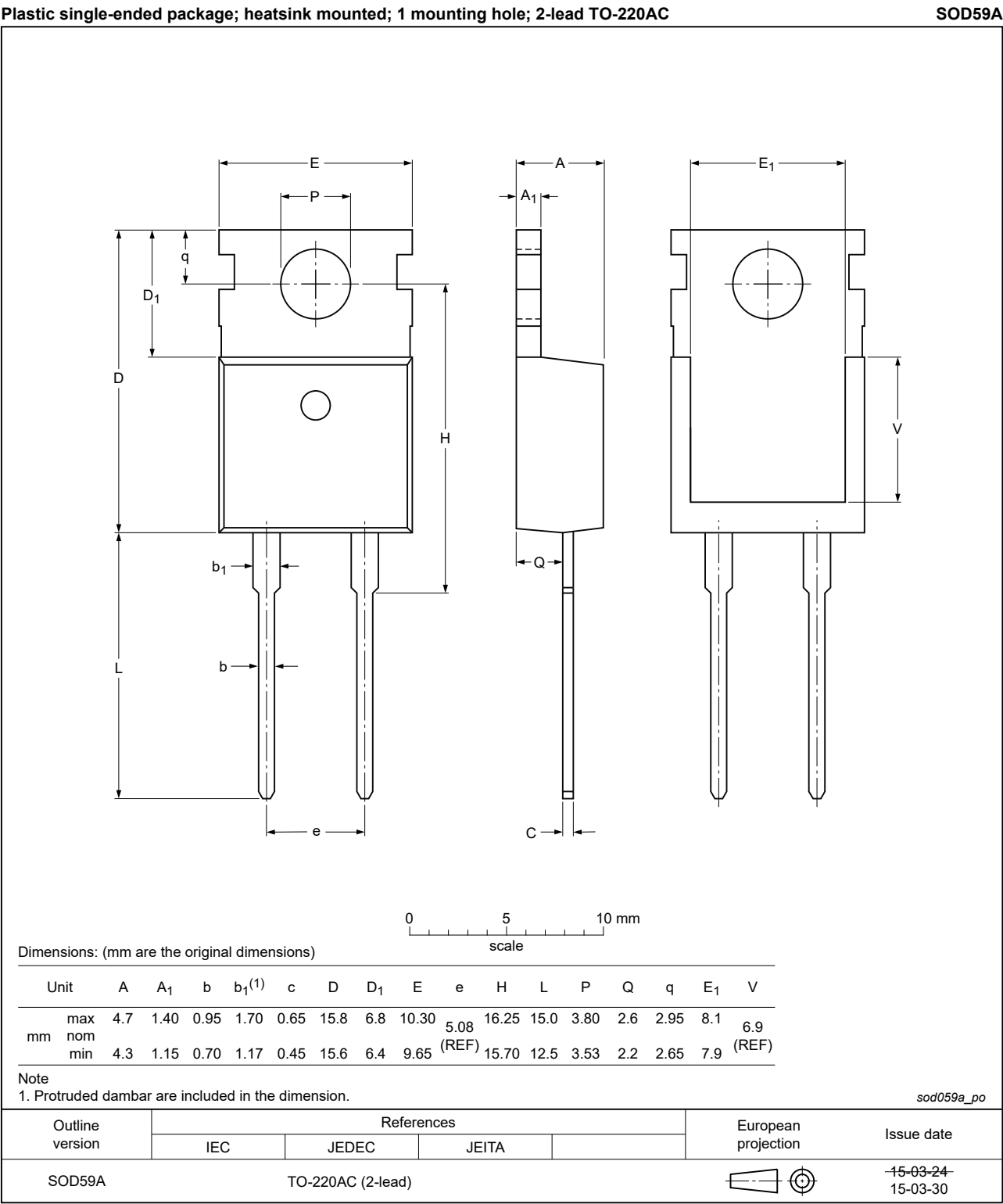
Fig. 7. Package outline TO-220AC (SOD59A)
