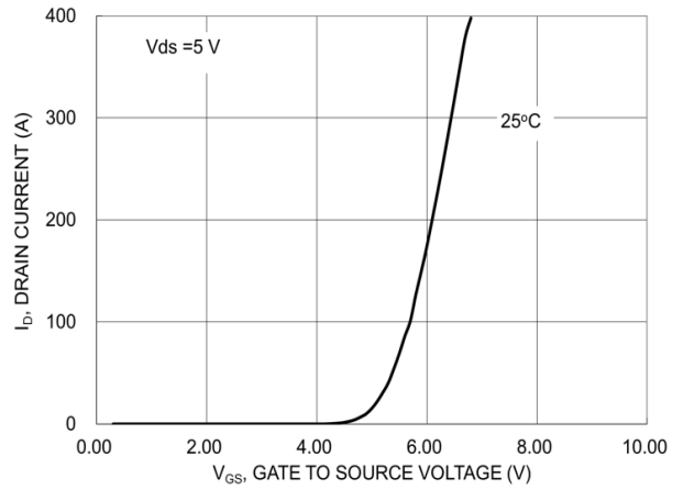
Figure 12. Transfer Characteristics
