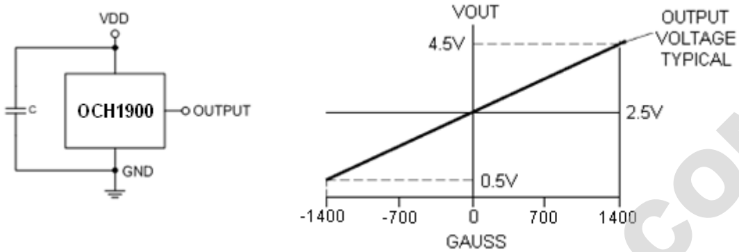
Figure 2, Typical Application of OCH1900
