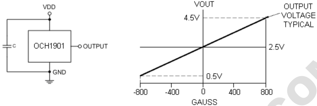
Figure 2, Typical Application of OCH1901
