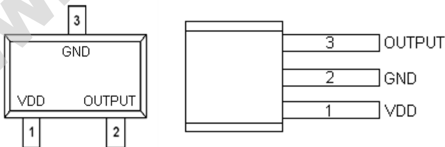
Figure 1, Pin Assignments of OCH1901
