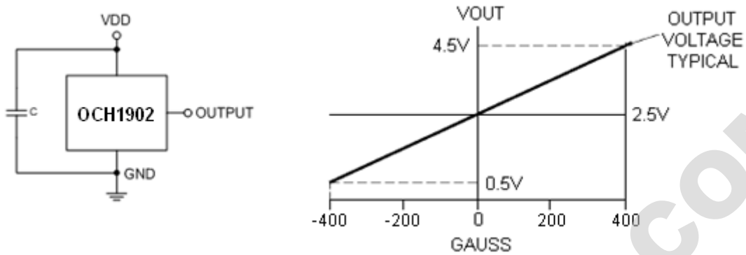
Figure 2, Typical Application of OCH1902
