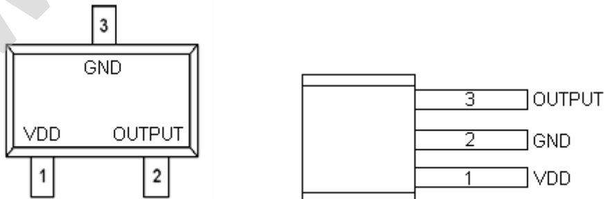
Figure 1, Pin Assignments of OCH1902
