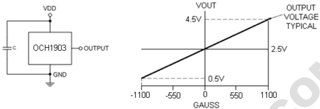
Figure 2, Typical Application of OCH1903
