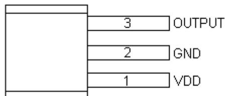
Figure 1, Pin Assignments of OCH1903
