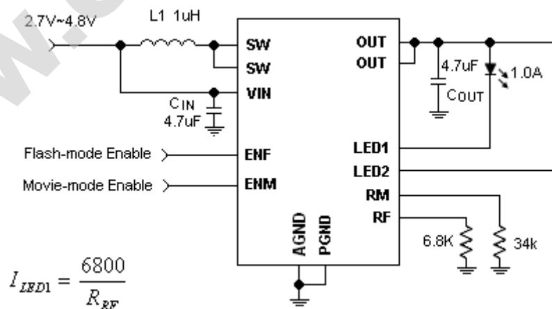
Figure 2C, Typical Application Circuit of OCP8132 (One Channel)
