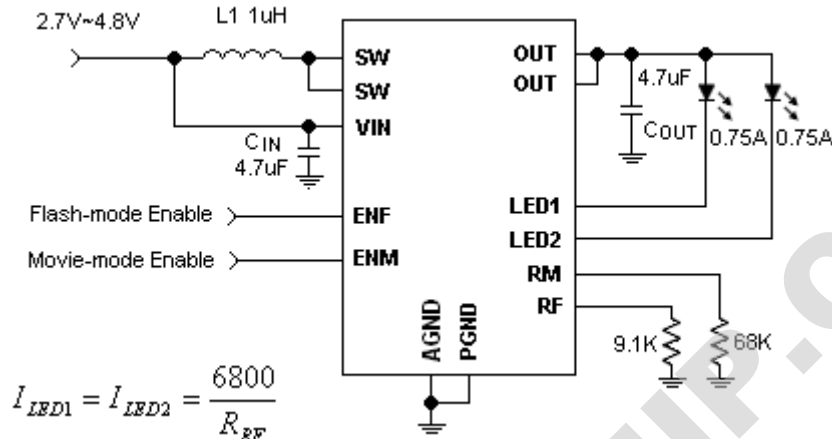
Figure 2A, Typical Application Circuit of OCP8132
