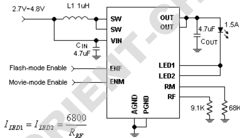
Figure 2B, Typical Application Circuit of OCP8132 (One Channel)
