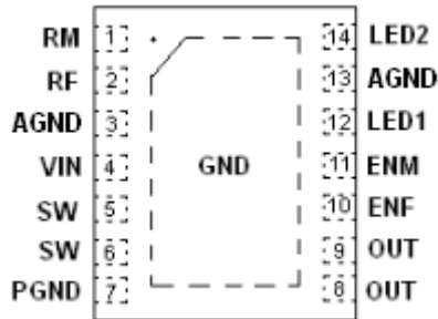
Figure 1, Pin Assignments of OCP8132
