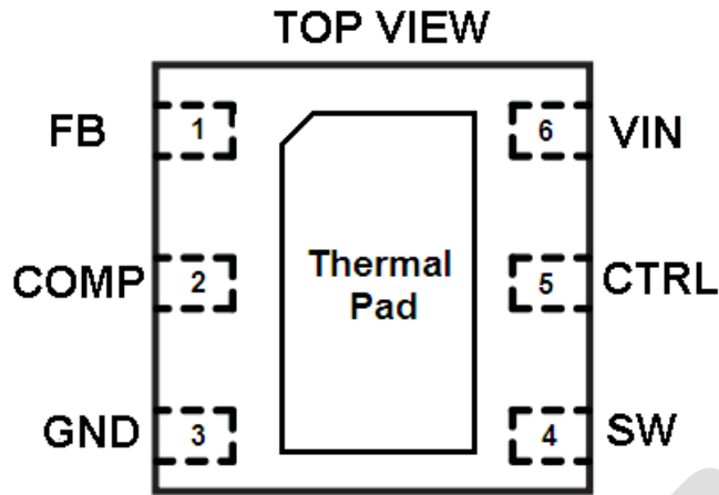
Figure 1, Pin Assignments of OCP8178
