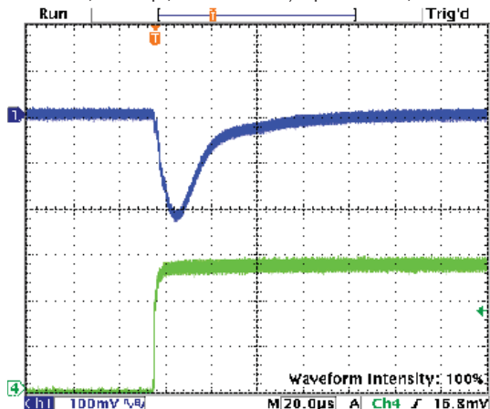
Step Load Transient Response (Vin=4.5V, Vout=1.8V, Cload=5x10µF X5R 0805 ceramic, total 50µF, Iout=0A to 1.5A) Top trace=Vout, Bottom trace=Iout
