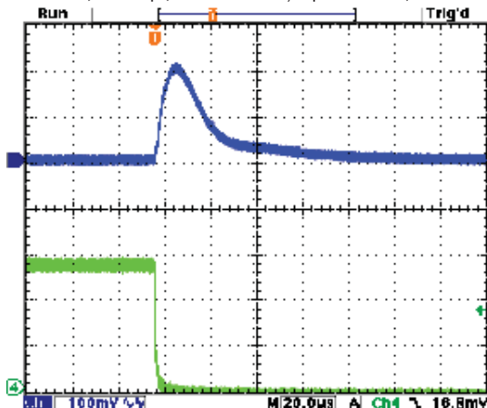
Step Load Transient Response (Vin=4.5V, Vout=1.8V, Cload=5x10µF X5R 0805 ceramic, total 50µF, Iout=1.5A to 0A) Top trace=Vout, Bottom trace=Iout
