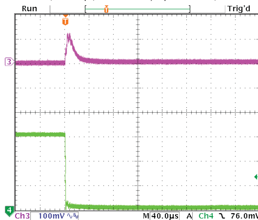
Step Load Transient Response (Vin=7.5V, Vout=5V, Cload=5x10µF X5R 0805 ceramic, total 50µF, Iout=3A to 0A) Top trace=Vout, Bottom trace=Iout
