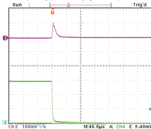
Step Load Transient Response (Vin=12V, Vout=5V, Cload=12x10µF X5R 0805 ceramic, total 120µF, Iout=3A to 0A) Top trace=Vout, Bottom trace=Iout
