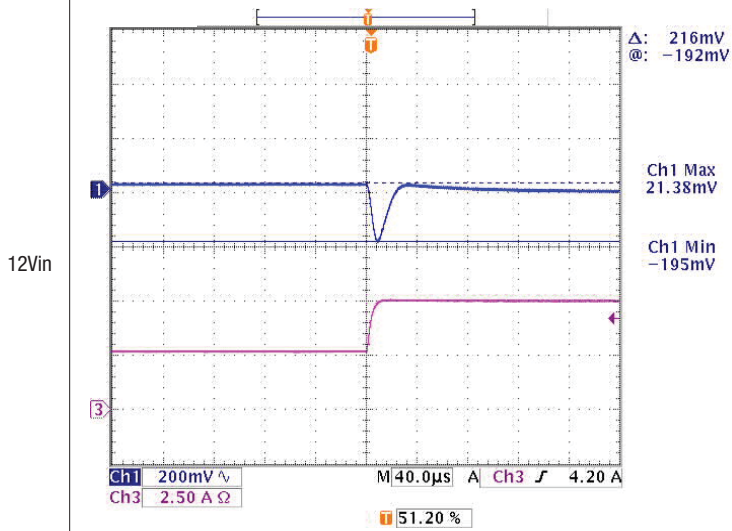
Step Load Transient Response (Vin=12V, Vout=5V, Load = 1 uF || 10 uF) Top trace=Vout, Bottom trace=Iout 2.5A → 5.0A
