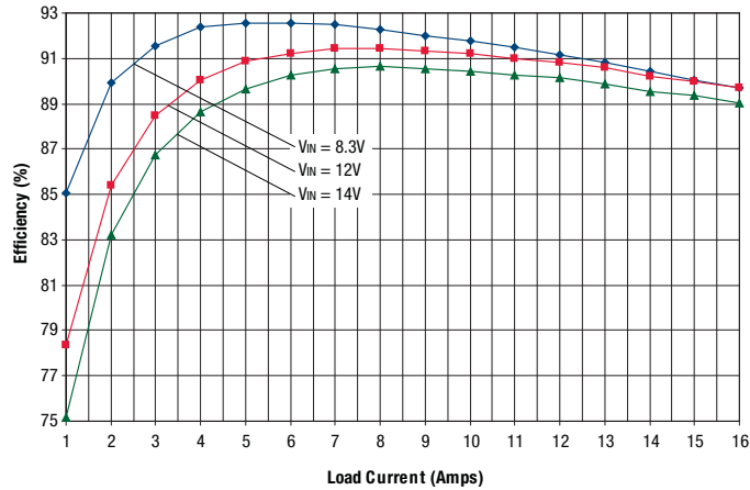
OKY2-T/16-D12 Efficiency vs. Line Voltage and Load Current @ +25°C (V OUT = 2.5V)
