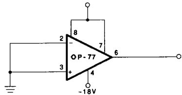
PINOUTS SHOWN FOR J, P, AND Z PACKAGES
