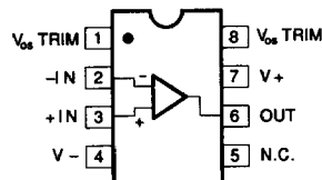
EPOXY MINI-DIP (P-Suffix)
