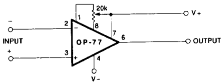
PINOUTS SHOWN FOR J, P, AND Z PACKAGES
