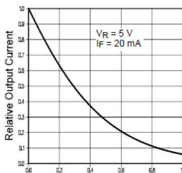
Coupling Characteristics OP905 and OP265
