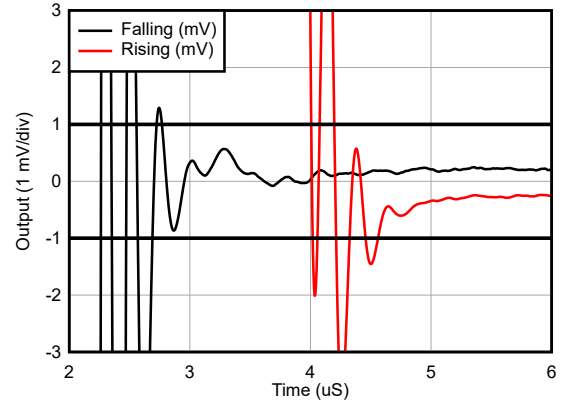
Figure 6-38. Settling Time
