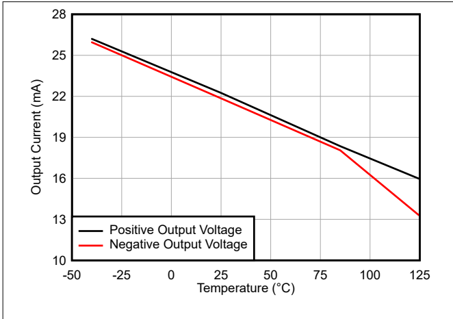
Figure 6-43. Short-Circuit Current vs Temperature
