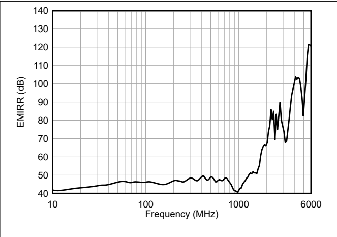
Figure 6-44. Electromagnetic Interference Rejection (EMIRR)
