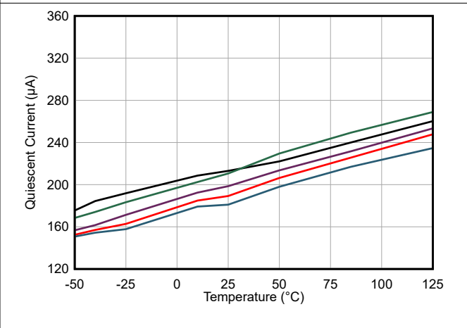
Figure 6-46. Quiescent Current vs Temperature
