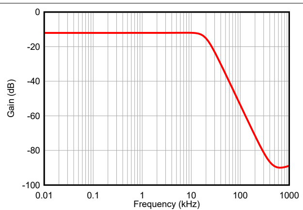
Figure 9-3. Attenuator + Filter Response
