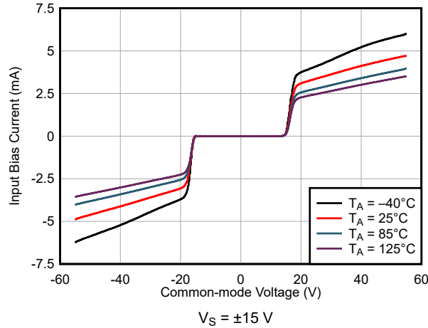
Figure 8-2. OPAx206 Input Current vs Input Voltage ( V_S = \pm 15\text{ V} )
