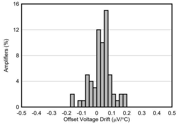
Figure 8-5. OPAx206 e-trim™ Operational Amplifier Drift
