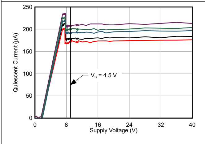
Figure 6-45. Quiescent Current vs Supply Voltage
