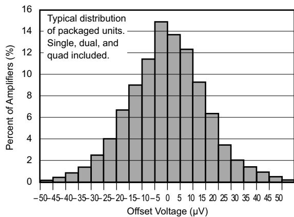
Figure 8-3. OPA2277 Laser-Trimmed Operational Amplifier Offset
