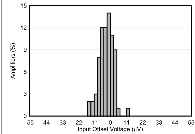
Figure 6-1. Offset Voltage Production Distribution at 25°C
