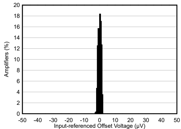
Figure 8-4. OPAx206 e-trim™ Operational Amplifier Offset
