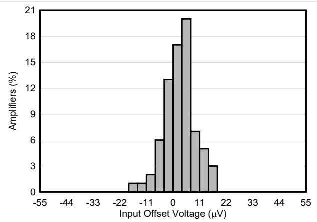
Figure 6-2. Offset Voltage Distribution at 125°C
