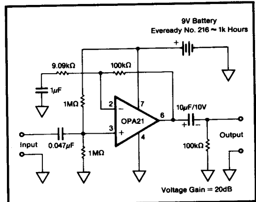
FIGURE 4. AC Amplifier.
