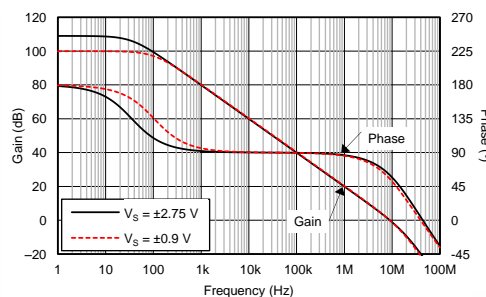
Low-Supply Current (400 μA/ch) for 10-MHz Bandwidth
