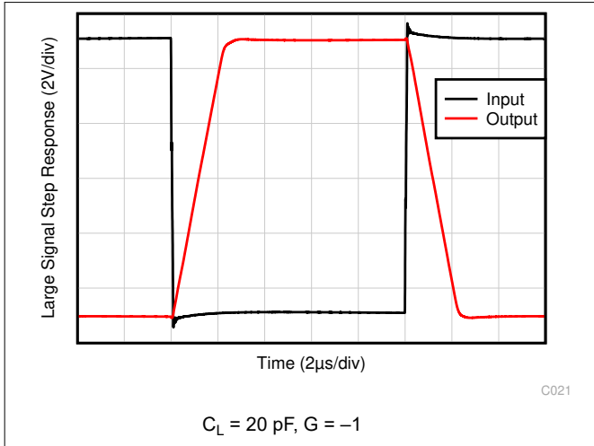
Figure 6-37. Large-Signal Step Response
