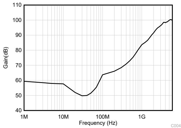
Figure 7-3. EMIRR Testing
