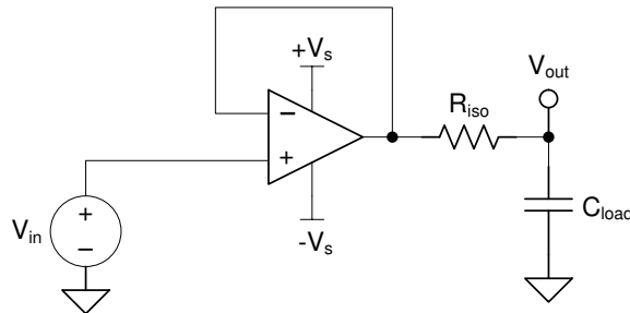
Figure 7-7. Extending Capacitive Load Drive With the OPAx991-Q1
