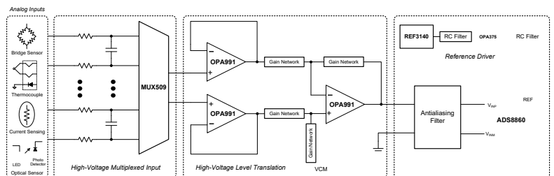
OPAx991-Q1 in a High-Voltage Signal Chain
