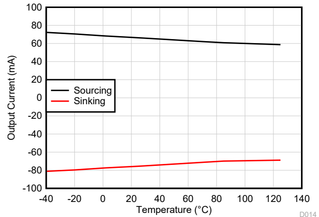
Figure 6-38. Short-Circuit Current vs Temperature D014
