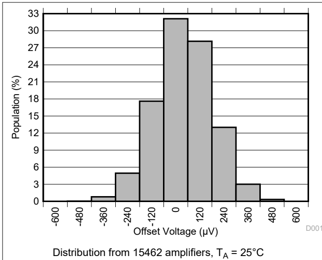
Figure 6-1. Offset Voltage Production Distribution
