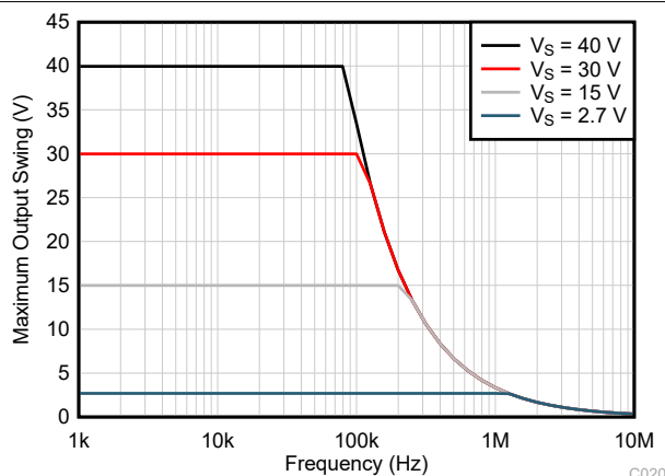
Figure 6-39. Maximum Output Voltage vs Frequency C020
