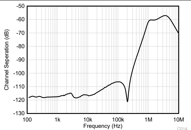
Figure 6-40. Channel Separation vs Frequency C014
