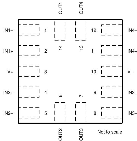
Figure 5-9. OPA4991 RTE Package (1)(2) 16-Pin WQFN With Exposed Thermal Pad Top View
