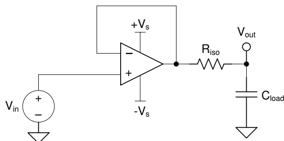
Figure 7-7. Extending Capacitive Load Drive With the OPA992-Q1
