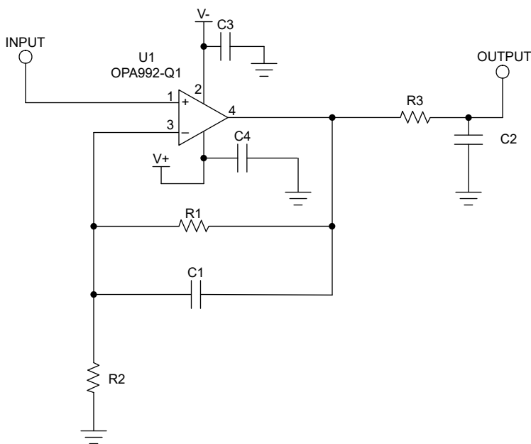
Figure 8-3. Schematic for Noninverting Configuration Layout Example
