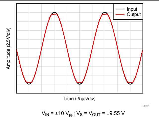
Figure 6-34. No Phase Reversal
