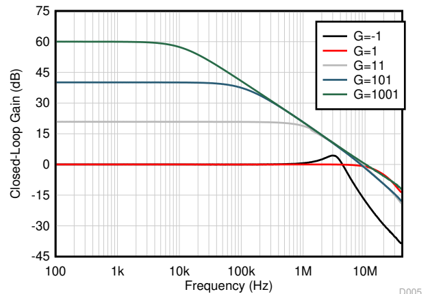
Figure 6-12. Closed-Loop Gain vs Frequency
