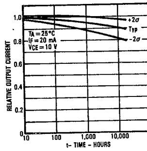
Relative Output Current vs Time
